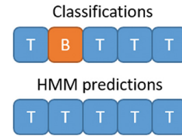
Fig. 6. Top row shows a sequence of Train and Bus classifications. They are corrected using HMM smoothing into a sequence of only Train activities shown below.
